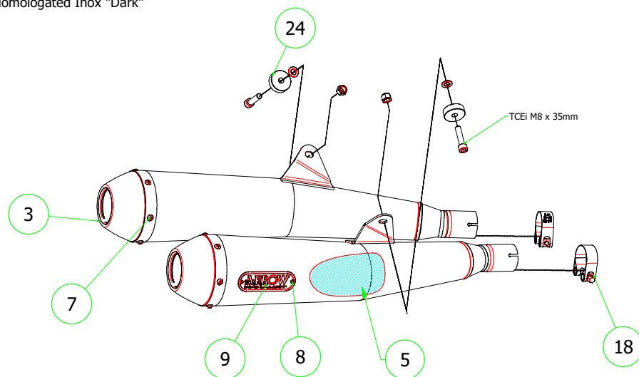
71851PRN Homologated Inox "Dark"
