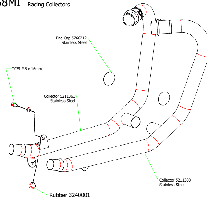
71658MI Racing Collectors
