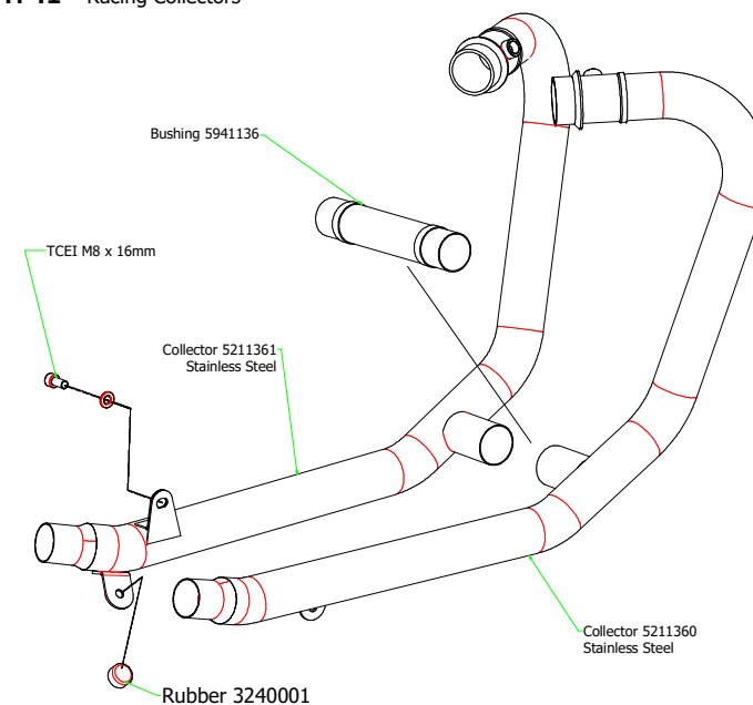
71664MI Racing Collectors
